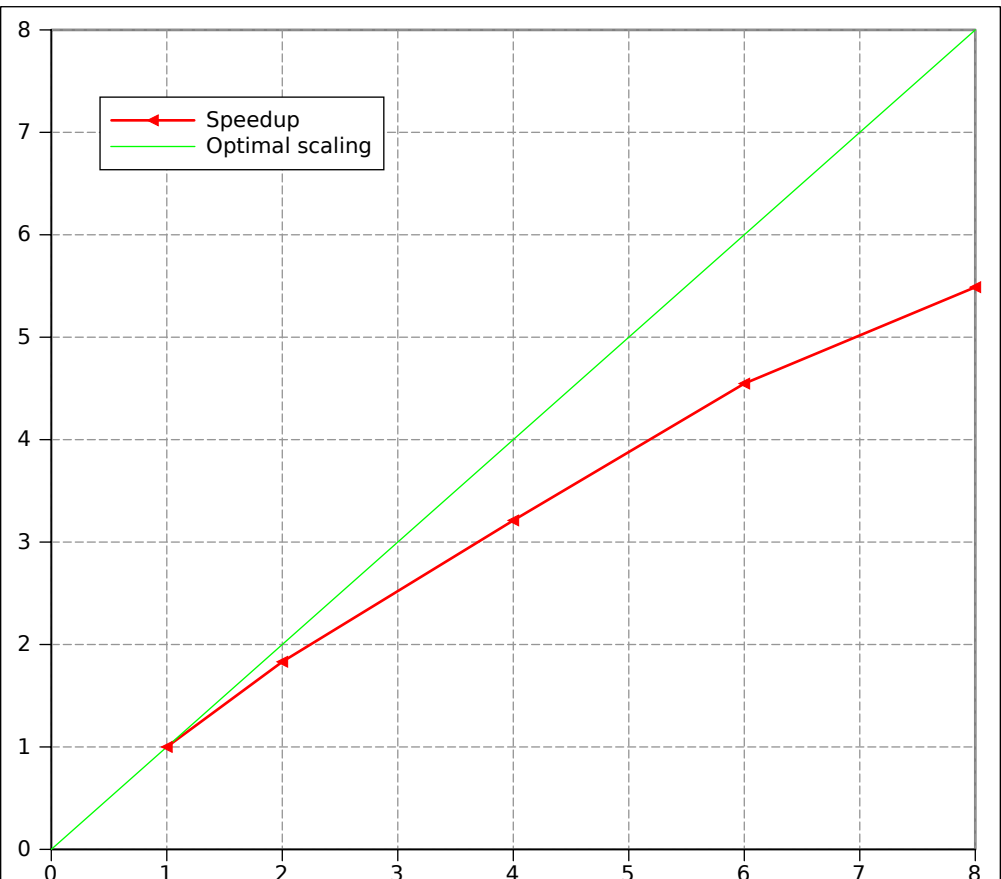
multicore scaling (OpenMP)
